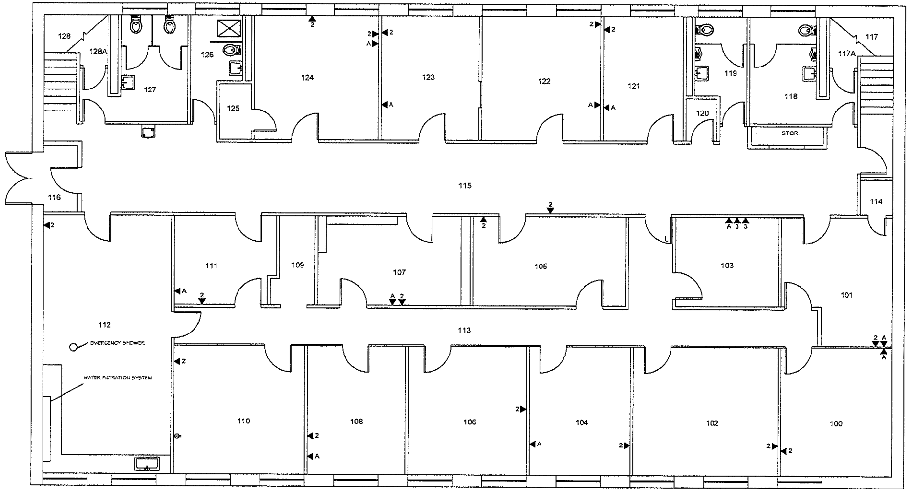
FIRST LEVEL FLOOR PLAN (LOWER) 4996.68 Gross SQFT
